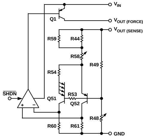
Figure 40. Simplified Schematic
