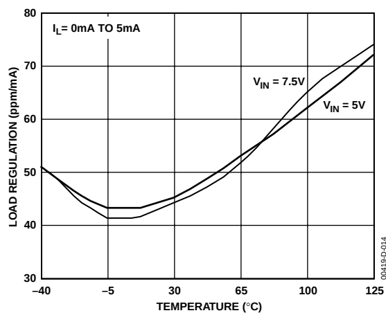
Figure 14. ADR395 Load Regulation vs. Temperature
