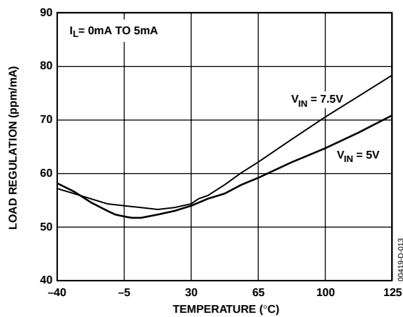
Figure 13. ADR392 Load Regulation vs. Temperature
