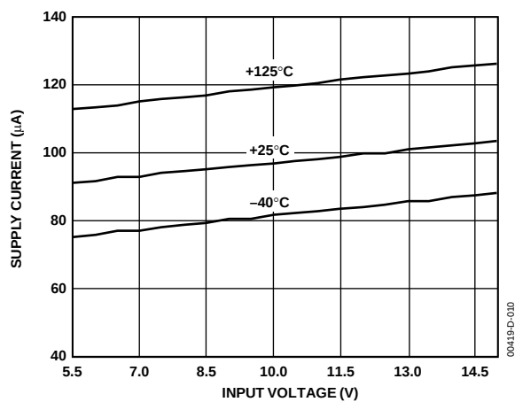
Figure 10. ADR395 Supply Current vs. Input Voltage
