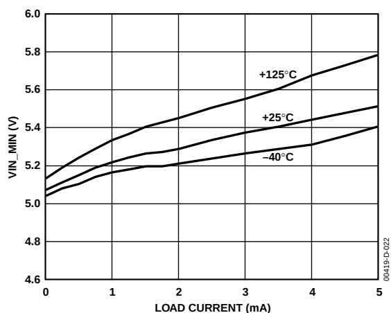
Figure 22. ADR395 Minimum Input Voltage vs. Load Current
