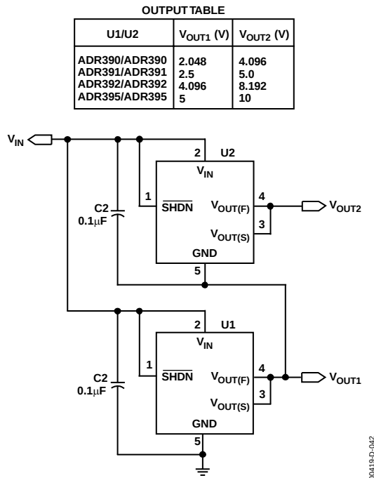
Figure 42. Stacking Voltage References with the ADR390/ADR391/ADR392/ADR395
