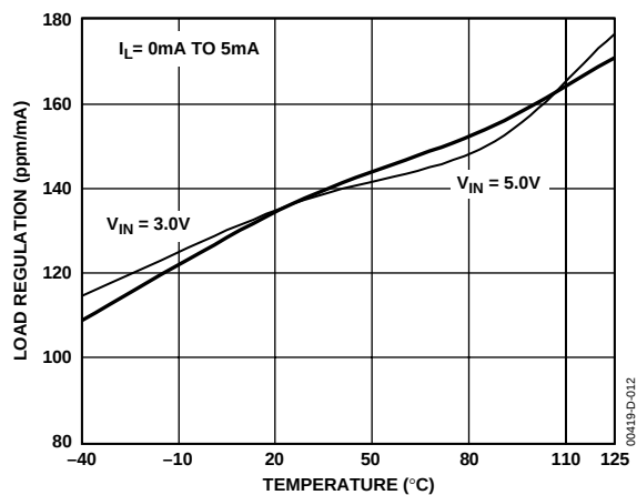
Figure 12. ADR391 Load Regulation vs. Temperature
