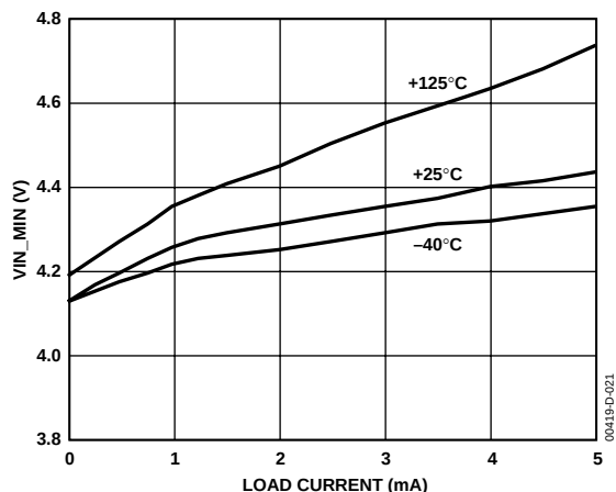
Figure 21. ADR392 Minimum Input Voltage vs. Load Current
