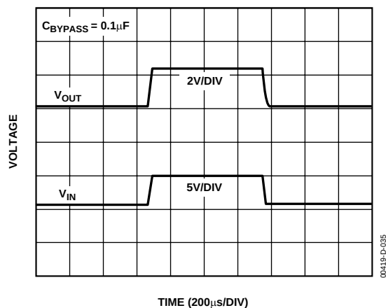
Figure 35. ADR391 Turn-On/Turn-Off Response at 5 V
