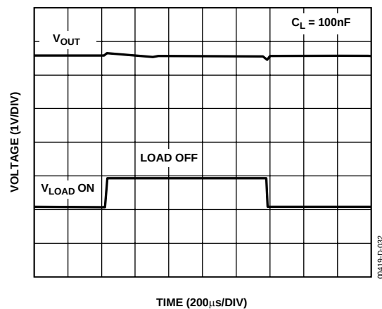
Figure 32. ADR391 Load Transient Response
