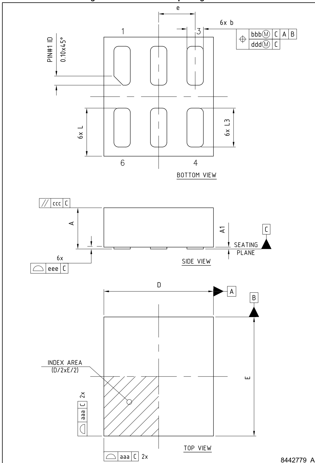
Figure 37. DFN6 1.2 x 1.3 package outline
