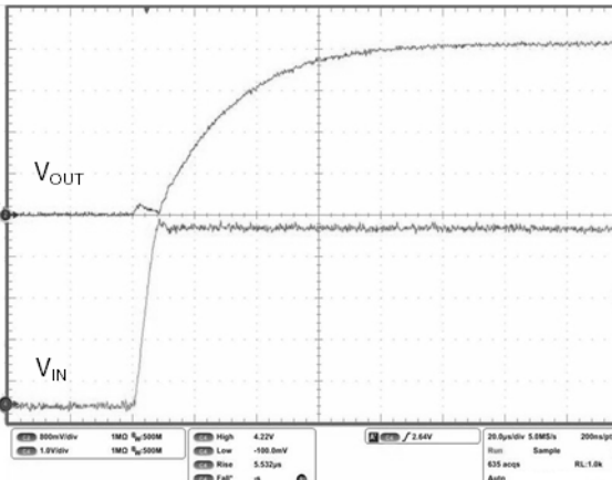
Figure 30. Startup transient
