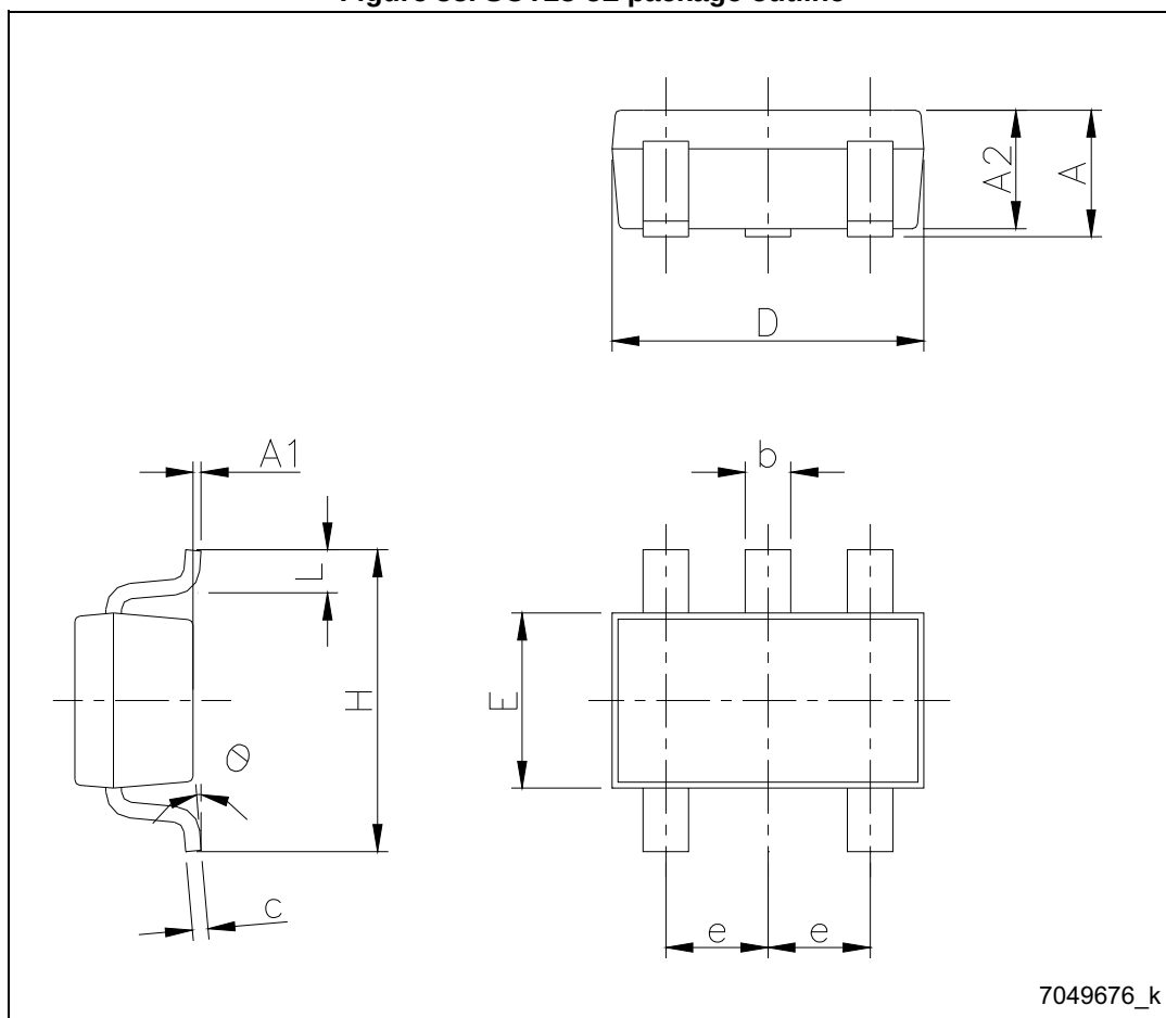
Figure 35. SOT23-5L package outline
