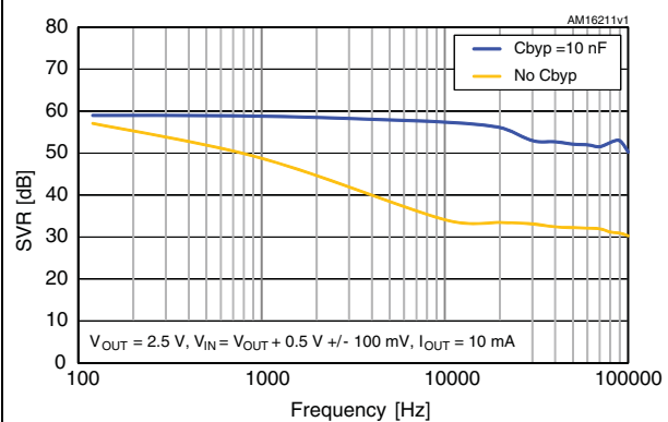
Figure 20. SVR vs. frequency ( V_O = 2.5 V)
