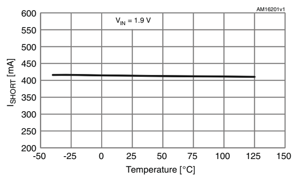
Figure 10. Short-circuit current vs. temp. for adjustable version
