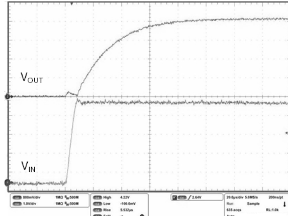
Figure 30. Startup transient
