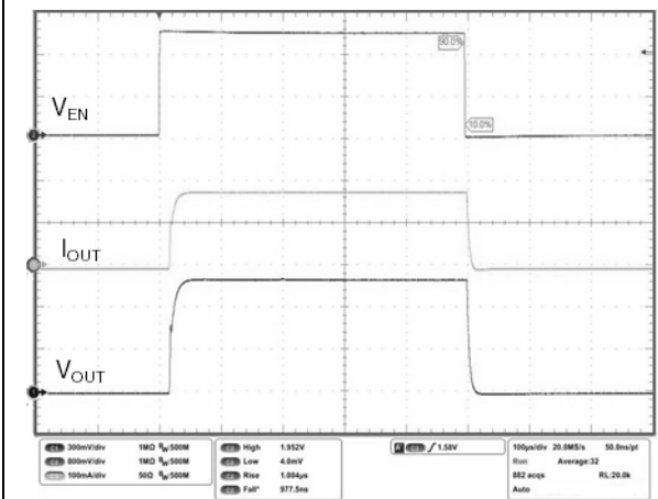
Figure 31. Enable transient ( V_{OUT} = V_{ADJ} )
