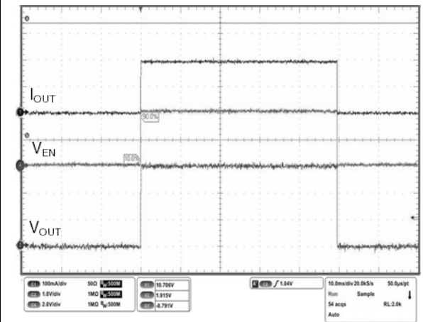
Figure 32. Enable transient ( V_{OUT} = 3 V)
