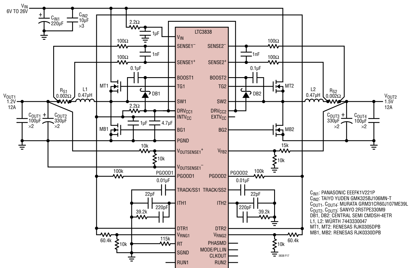
Figure 17. 6V to 26V Input, 1.2V/15A and 1.5V/15A Dual Output, 350kHz, R_{SENSE} , Step-Down Converter
