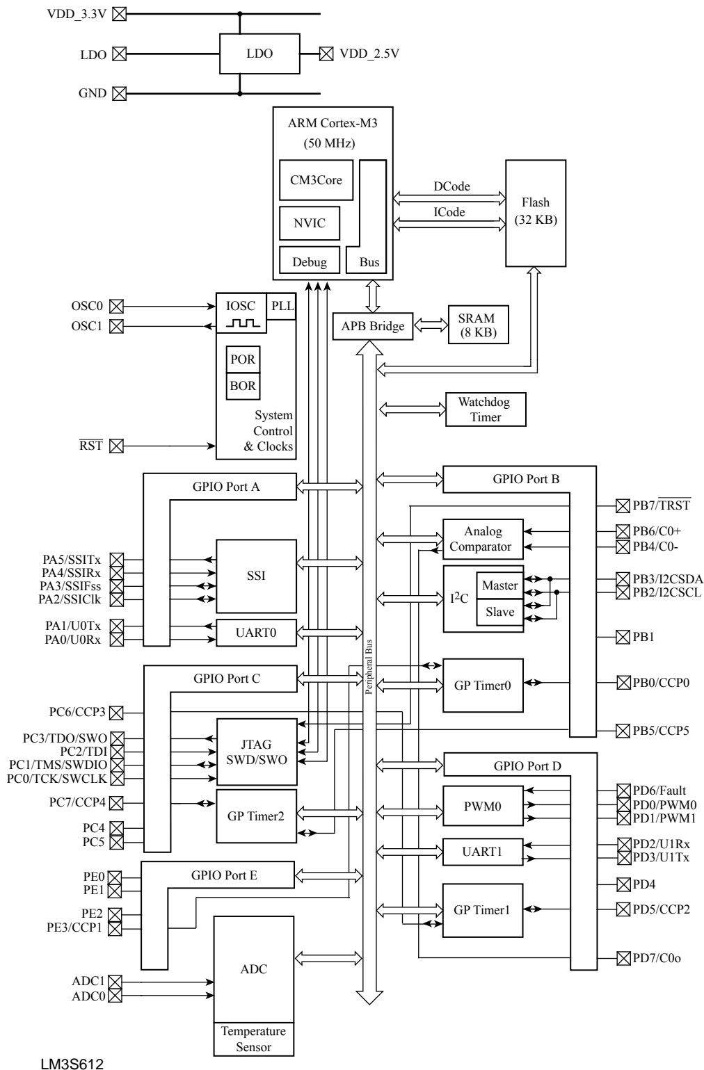
Figure 1-2. LM3S612 Controller System-Level Block Diagram
