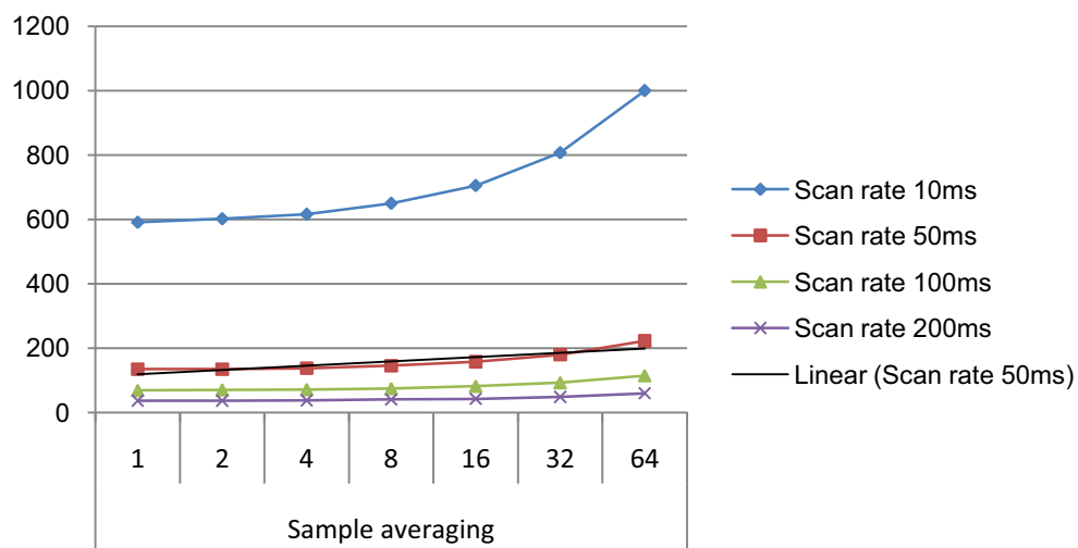
Figure 32-9. Power consumption [ \mu\text{A} ].
