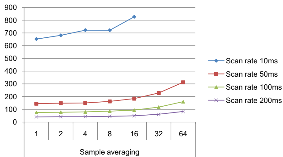
Figure 32-10. Power consumption [ \mu\text{A} ].
