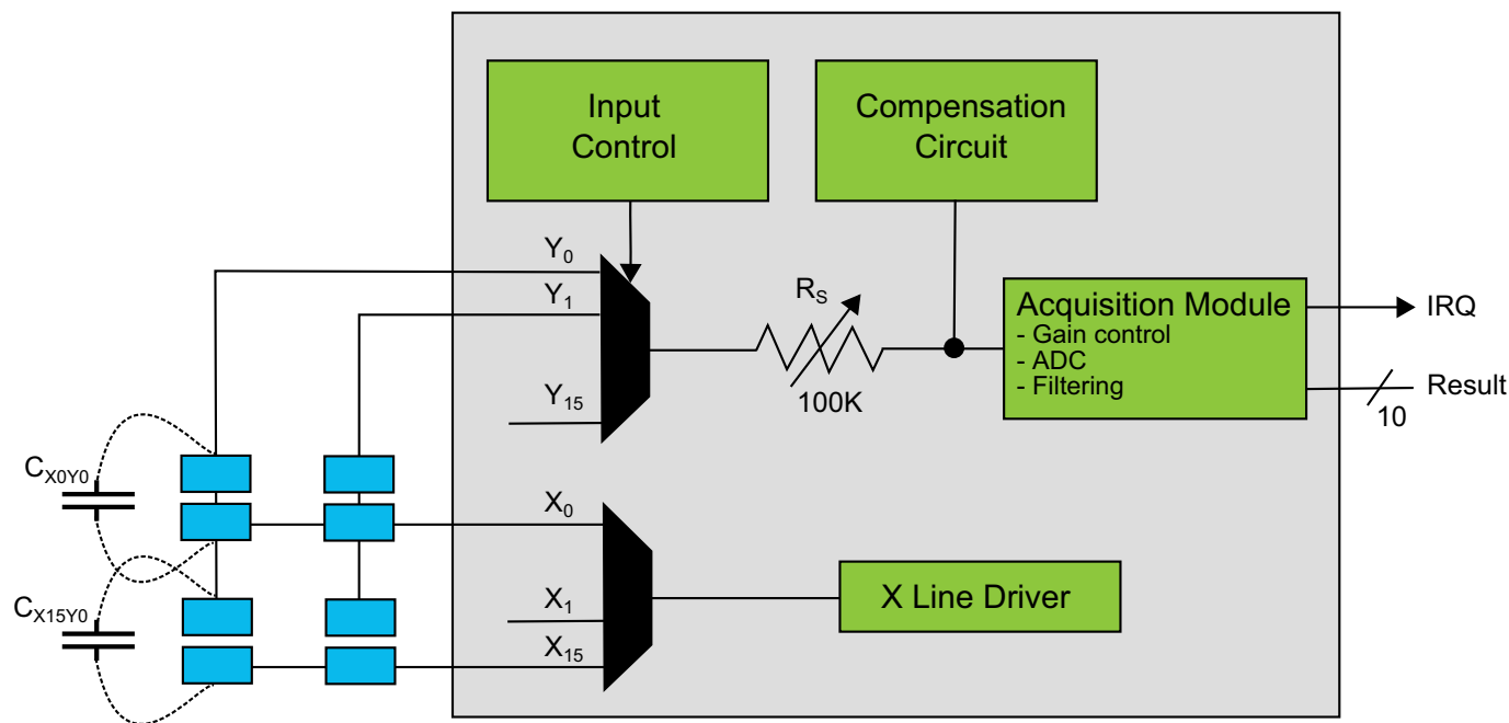
Figure 31-1. PTC Block Diagram Mutual-capacitance
