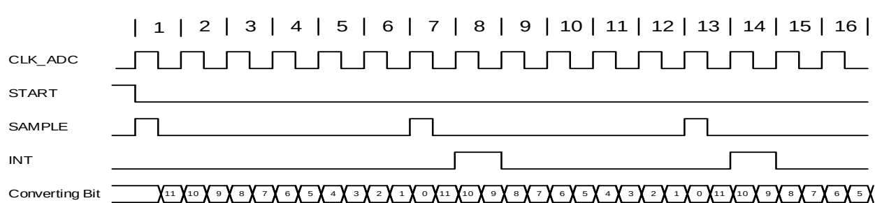
Figure 28-5. ADC Timing for Free Running in Differential Mode without Gain
