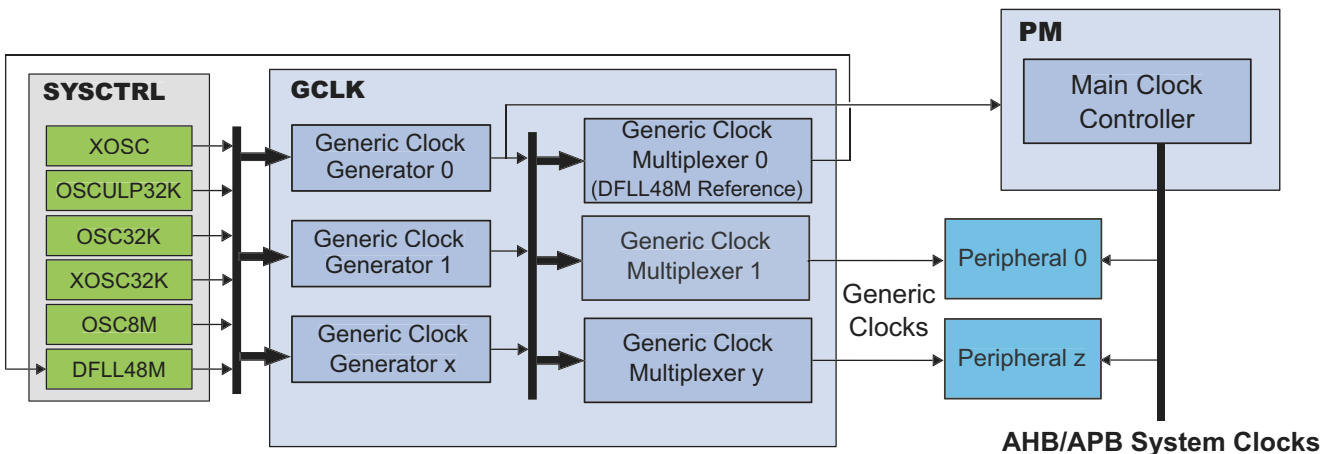
Figure 13-1. Clock distribution
