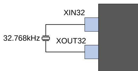
Figure 34-7. External Real Time Oscillator without Load Capacitor
