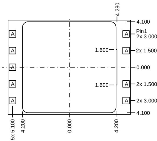
A= 0.600 x 0.600 mm BOTTOM PIN VIEW
