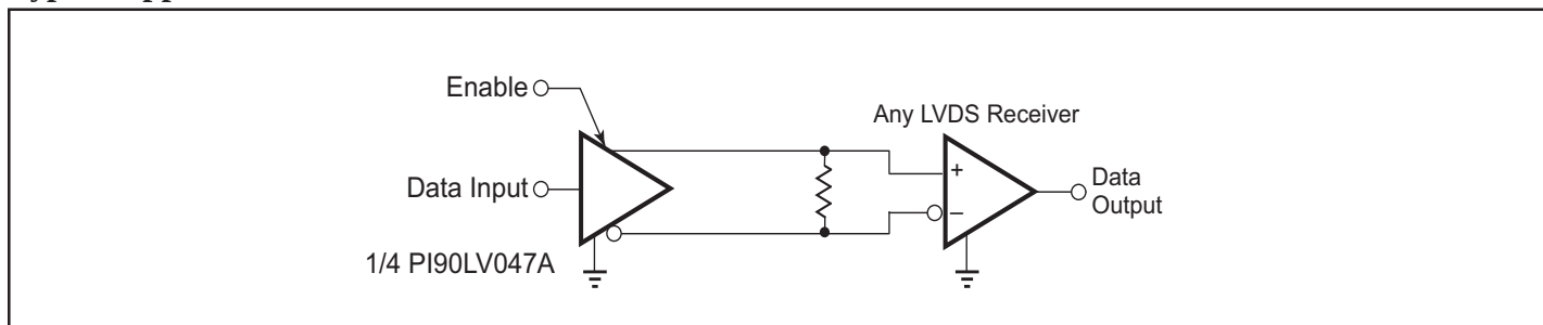
Figure 6. Point-to-Point Application
