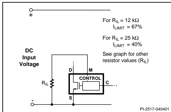
Figure 17. Externally Set Current Limit.
