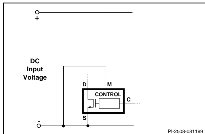
Figure 13. Three Terminal Operation (MULTI-FUNCTION Features Disabled. FREQUENCY Pin Tied to SOURCE or CONTROL Pin).
