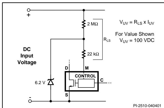
Figure 15. Line Sensing for Under-Voltage Only (Overvoltage Disabled).
