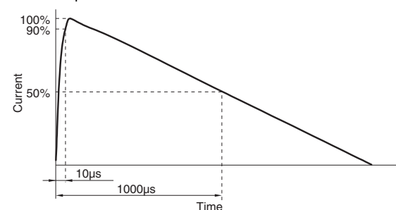
*2 10/1000µs test waveform
