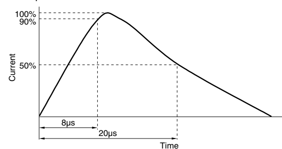
*1 8/20µs test waveform
