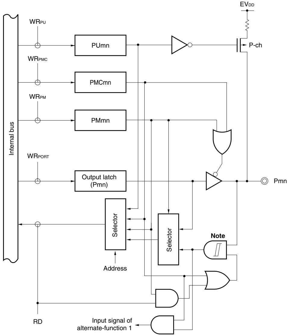
Figure 4-9. Block Diagram of Type D-1-2
