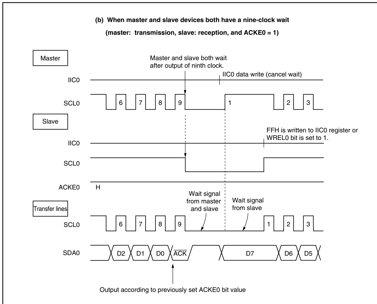
Figure 19-10. Wait Signal (2/2)
