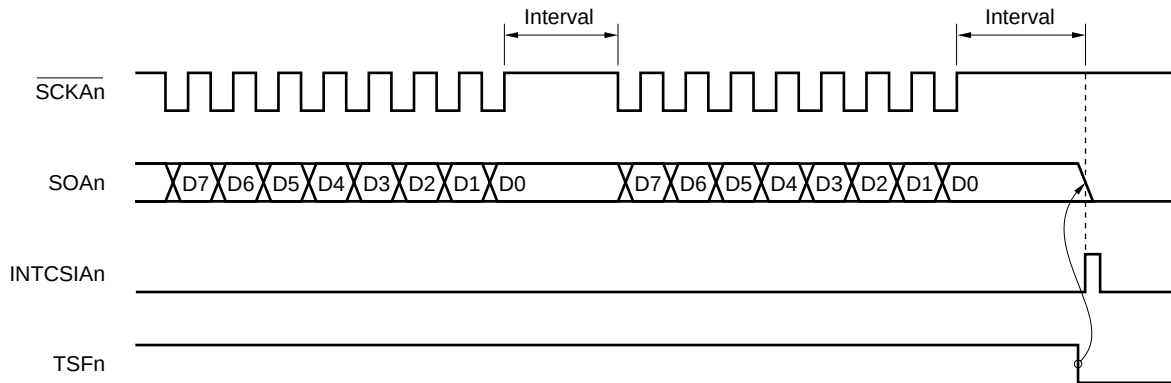
Figure 18-8. Automatic Transmission Mode Operation Timing
