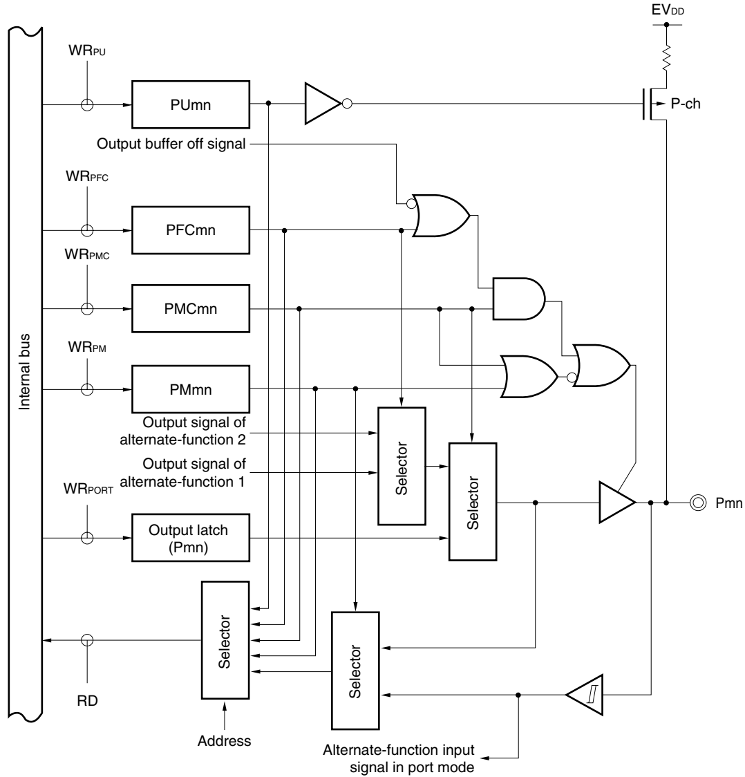
Figure 4-13. Block Diagram of Type E-3
