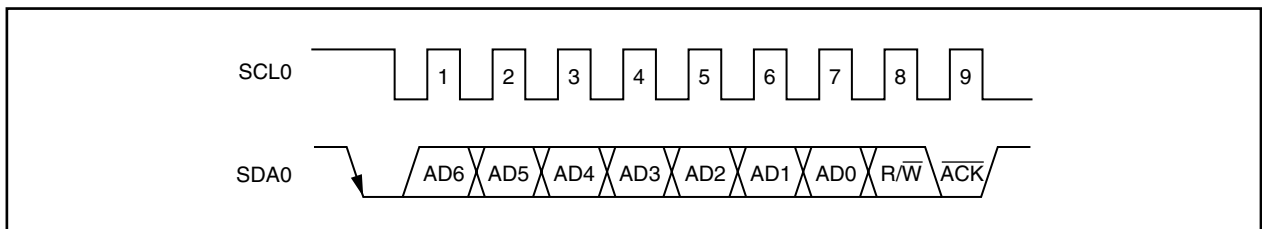
Figure 19-8. Acknowledge Signal ( \overline{\text{ACK}} )
