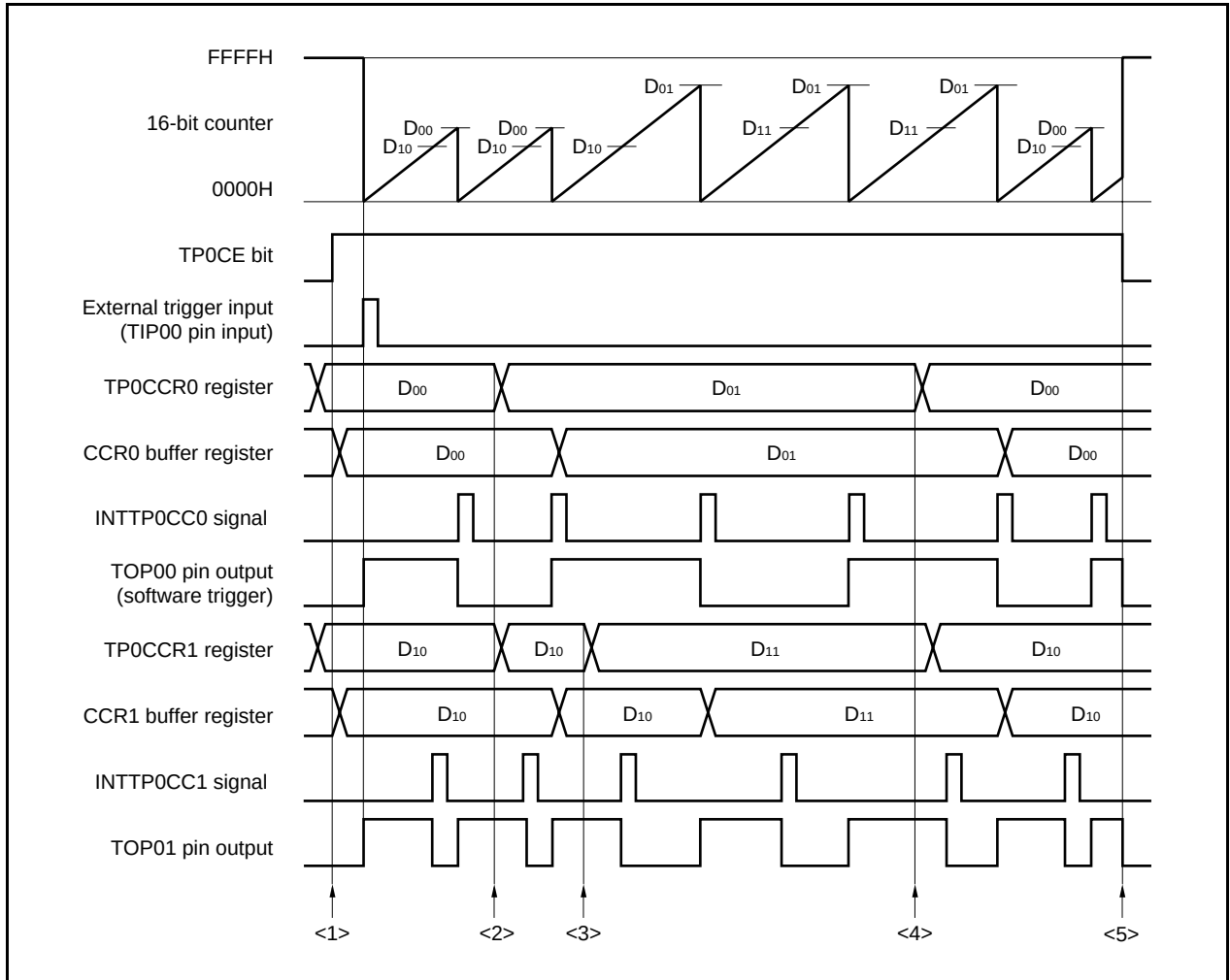
Figure 7-19. Software Processing Flow in External Trigger Pulse Output Mode (1/2)
