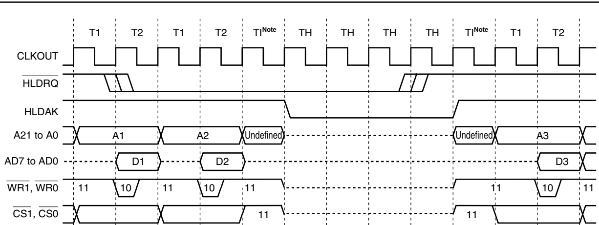
Figure 5-13. Separate Bus Hold Timing (Bus Size: 8 Bits, Write)
