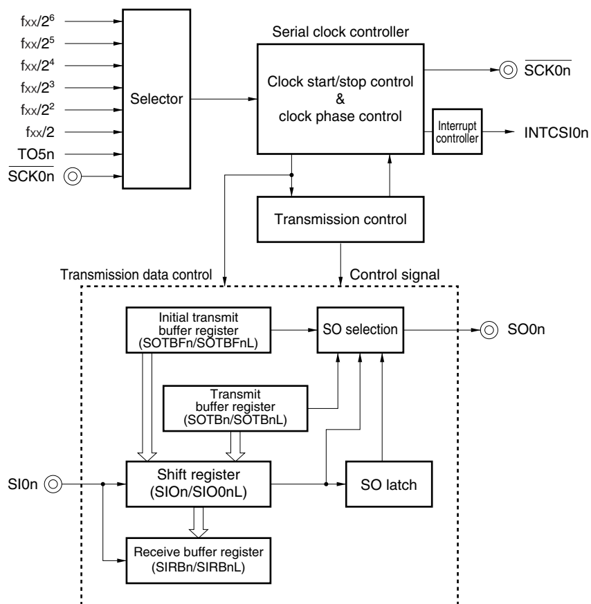
Figure 17-1. Block Diagram of Clocked Serial Interface
