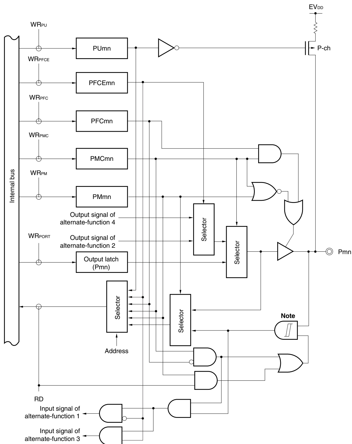
Figure 4-23. Block Diagram of Type G-7-1
