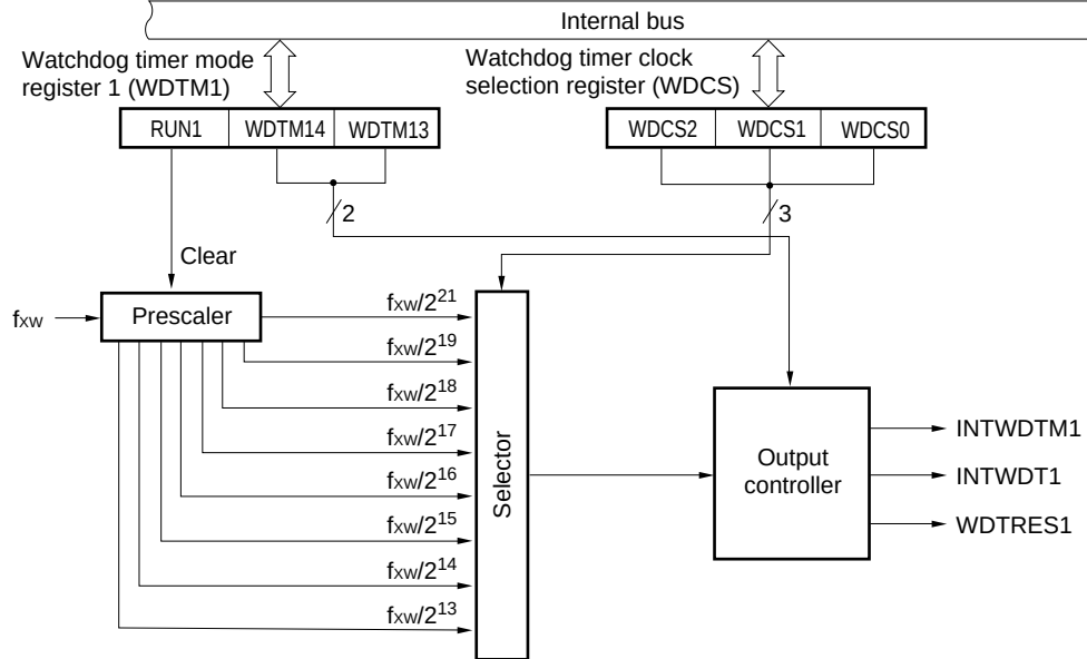
Figure 12-1. Block Diagram of Watchdog Timer 1
