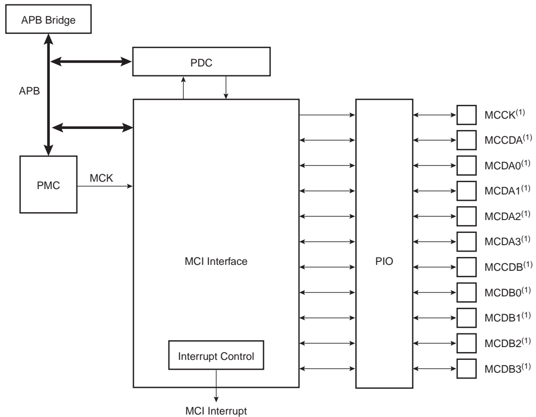
Figure 37-1. Block Diagram
