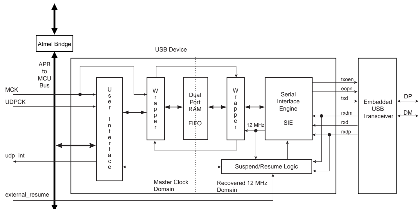
Figure 39-1. Block Diagram
