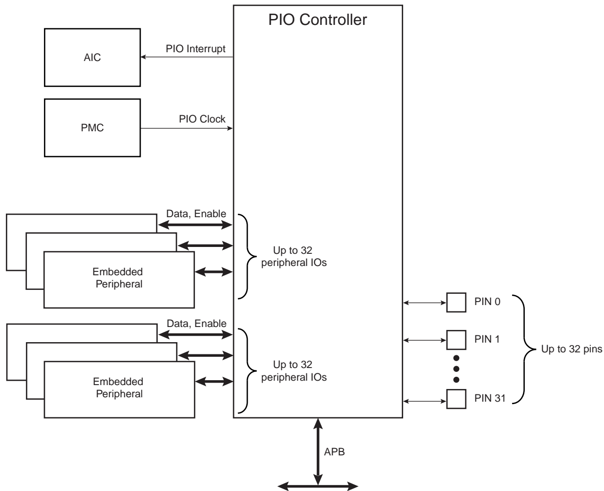
Figure 31-1. Block Diagram
