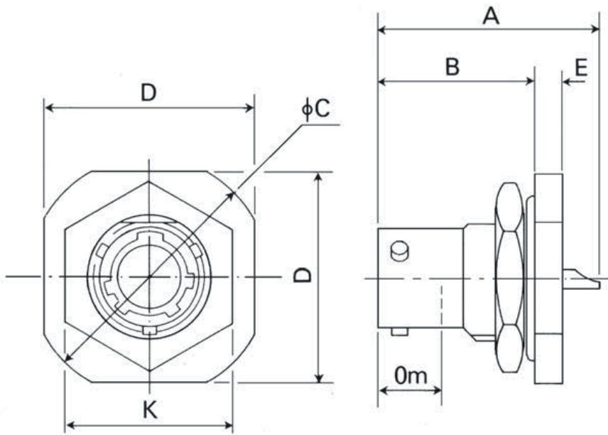
Panel Cut Out Dimensions
