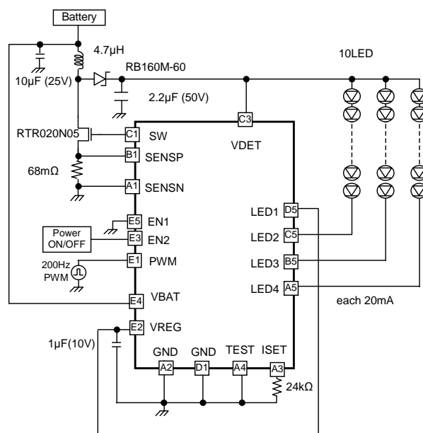
Fig.26 LED current 20mA setting example (10 series × 3parallel)
