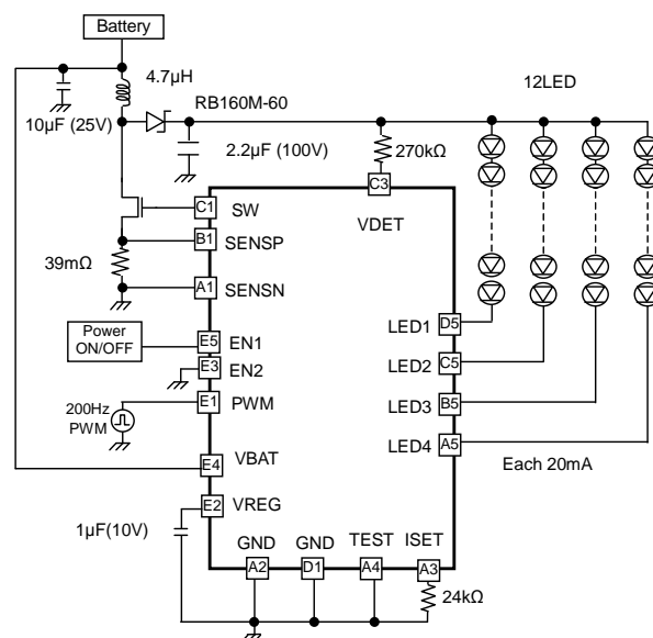
Fig.28 Over voltage 48.1V(typ) by external resistor, LED current 20mA setting example (12 series ( V_f=3.6V_{max} ) × 4parallel)
