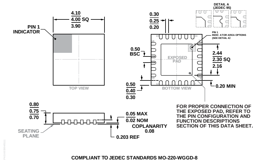
COMPLIANT TO JEDEC STANDARDS MO-220-WGGD-8 Figure 61. 24-Lead Lead Frame Chip Scale Package [LFCS] 4 mm × 4 mm Body and 0.75 mm Package Height (CP-24-14) Dimensions shown in millimeters
