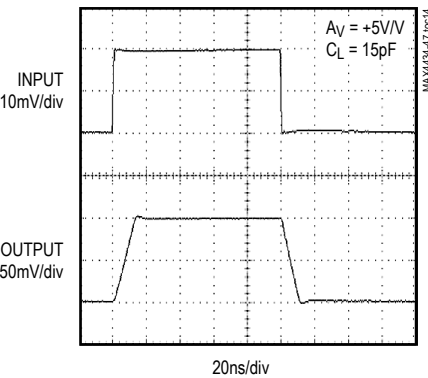
MAX4435/MAX4437 SMALL-SIGNAL PULSE RESPONSE
