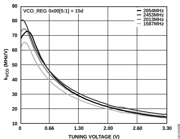
Figure 29. Typical VCO Sensitivity ( k_{VCO} )
