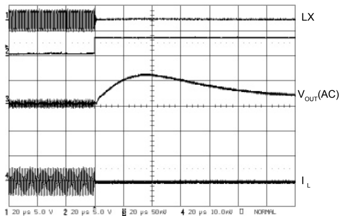
Handover Transition Switcher to Linear
