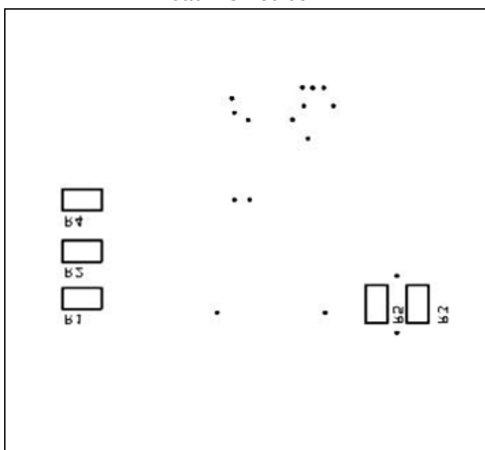
Bottom Silkscreen
