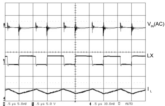
Input Voltage Ripple (FELDO active)
