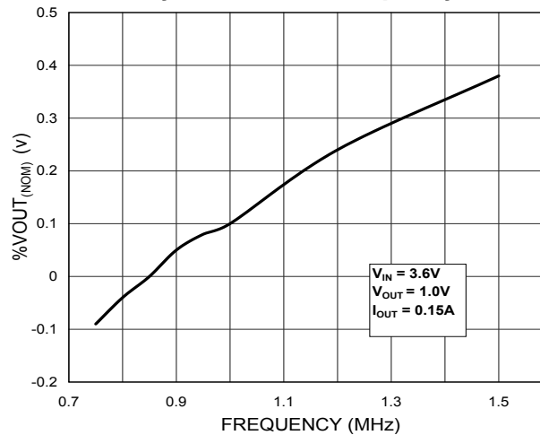
Output Voltage vs Synchronization Frequency
