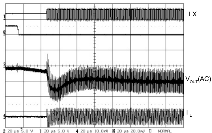
Handover Transition Linear to Switcher
