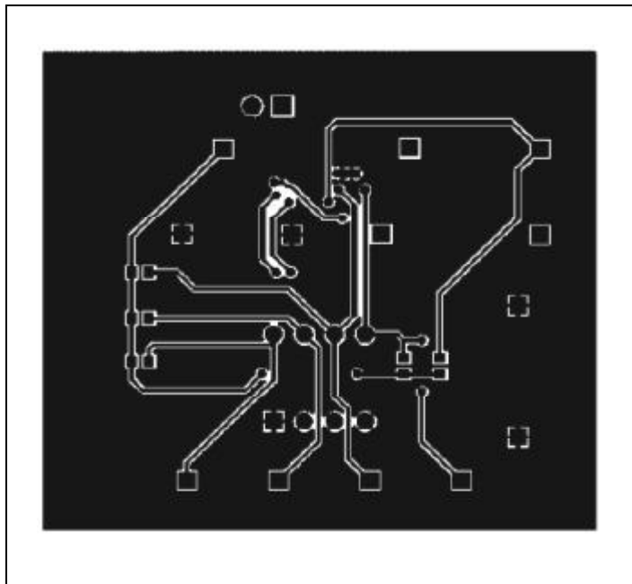
Bottom Copper
