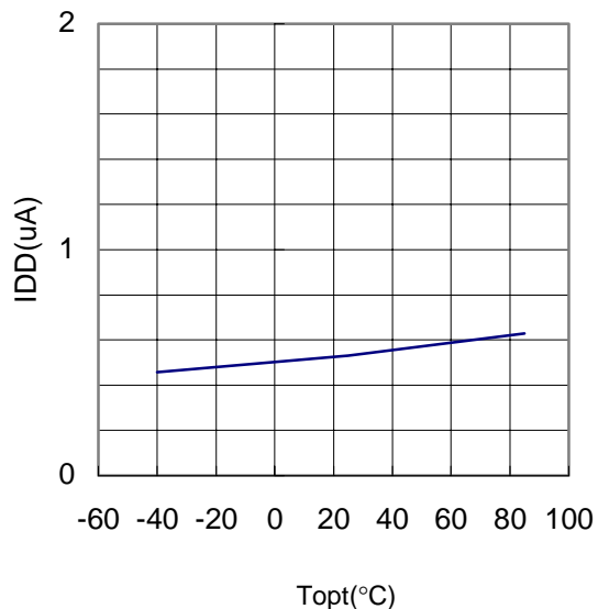
3.4. Stand-by Current vs. Temperature (VDD=3.0V, SDA=OPEN)
