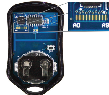
Figure 6: Address Traces
