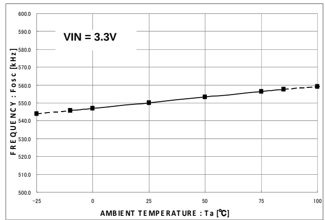
Fig.15 Switching frequency-temperature characteristic
