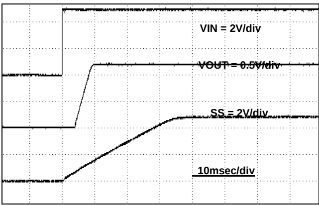
Fig.10 Soft start
