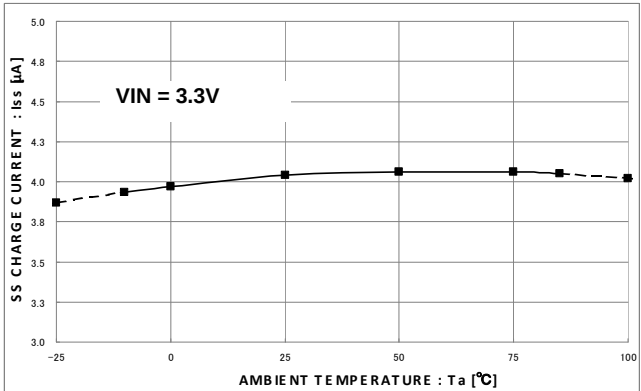
Fig.13 SS Charging current - Temperature characteristic
