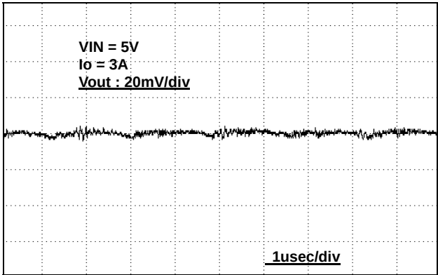
Fig.8 Output ripple
