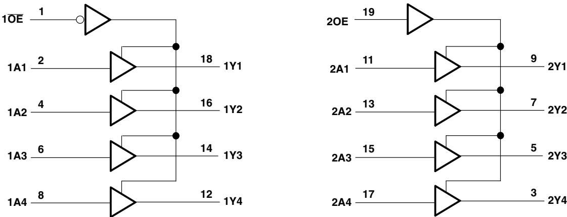
logic diagram (positive logic)
