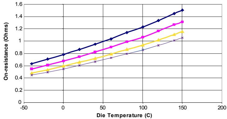
Lx on-resistance vs die temperature
