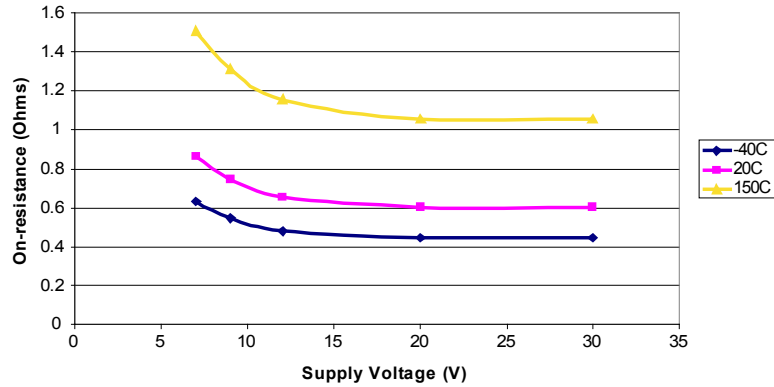
Lx on-resistance vs supply voltage
