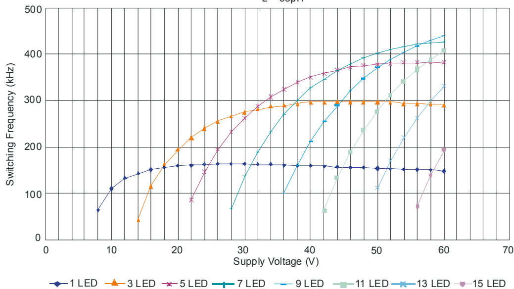
ZXLD1362 Switching Frequency L = 68\mu\text{H}
