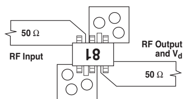
Figure 13. RF Layout.
