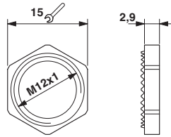
Dimensional drawing
