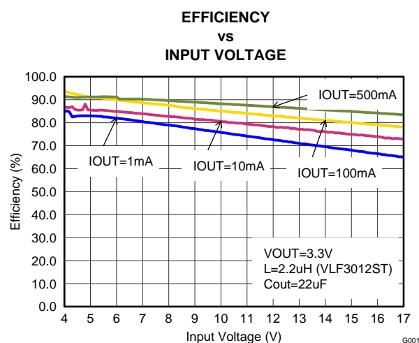
Figure 8. Vout=3.3V
