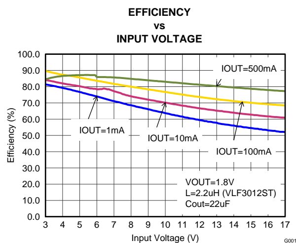
Figure 10. Vout=1.8V
