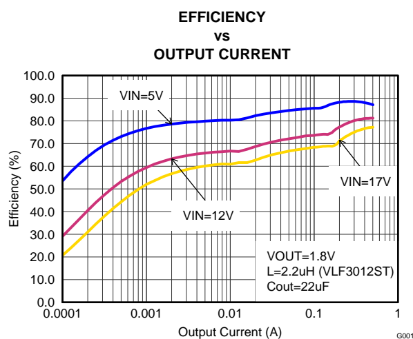
Figure 9. Vout=1.8V
