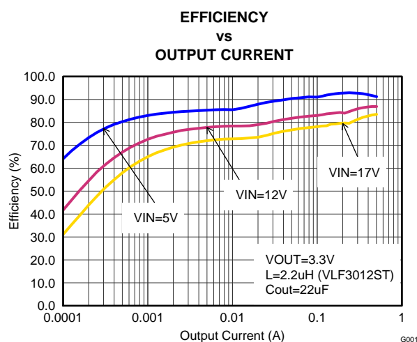
Figure 7. Vout=3.3V
