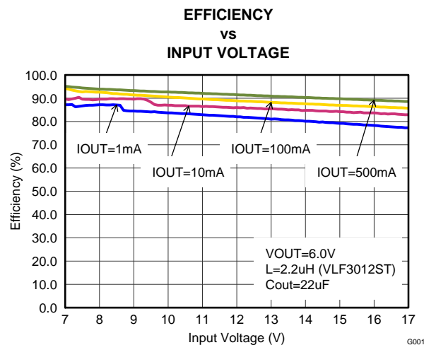
Figure 6. Vout=6V
