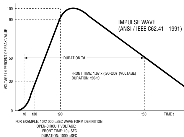
Figure 2. Surge Waveform
