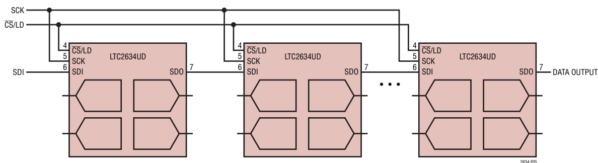
Figure 5. Daisy-Chain Operation (QFN Only)
