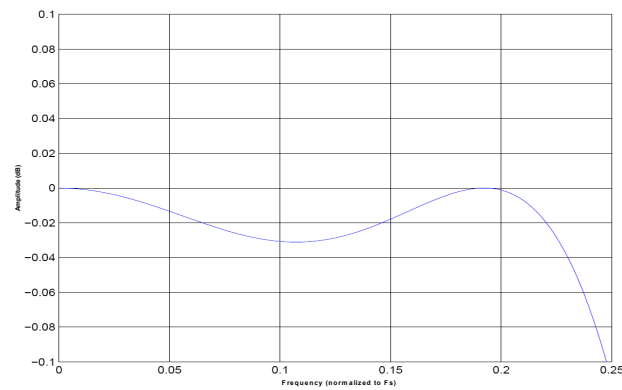
Figure 12. Quad-Speed Mode Passband Ripple
