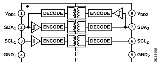
Figure 2. ADuM1251
