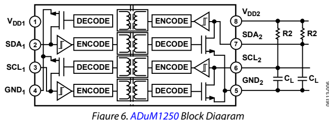
Figure 6. ADuM1250 Block Diagram
