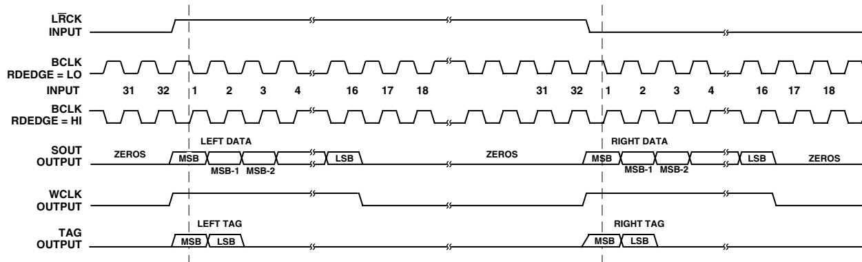
Figure 9. Serial Data Output Timing: Slave Mode, Left-Justified with No MSB Delay, \overline{S\overline{M}} = HI , \overline{RLJUST} = LO , \overline{MSBDLY} = HI
