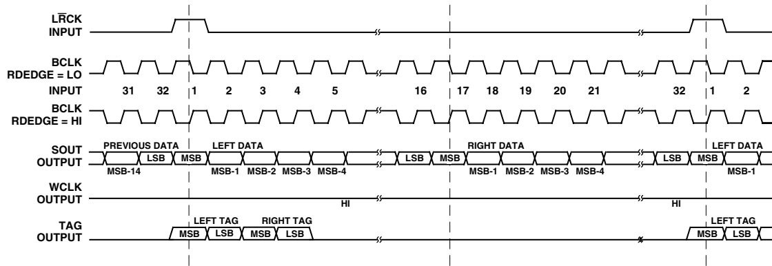
Figure 15. Serial Data Output Timing: Slave Mode, Left-Justified with No MSB Delay, 32-Bit Frame Mode, S/M = HI , RLJUST = LO , MSBDLY = HI
