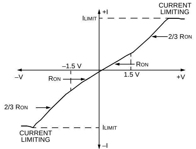
Figure 5. Switches 1—3
