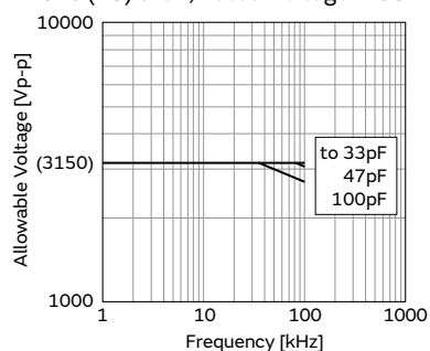
U2J (7U) char., Rated Voltage: DC3.15kV
