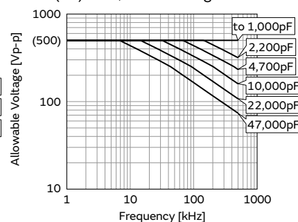
U2J (7U) char., Rated Voltage: DC500V
