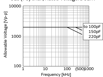
U2J (7U) char., Rated Voltage: DC2kV
