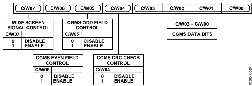
Figure 51. CGMS_WSS Register 0
