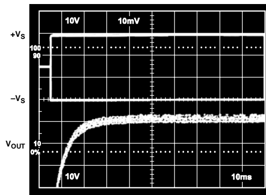
Figure 11. Turn-On with CN = 1 \mu F
