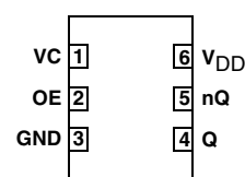
IDT8N4SV75 6-lead ceramic 5mm x 7mm x 1.55mm package body CD Package Top View
