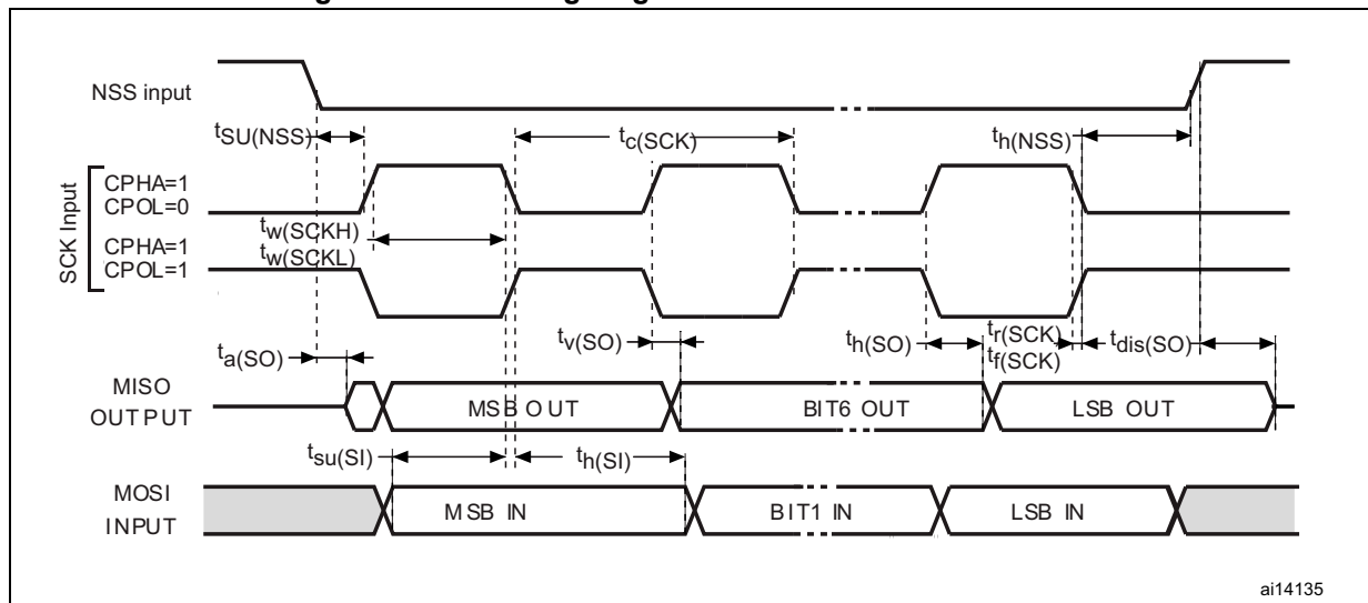
Figure 46. SPI timing diagram - slave mode and CPHA = 1
