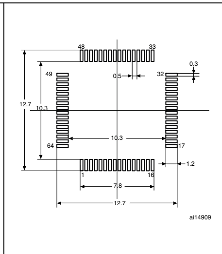
Figure 36. Recommended footprint (1)(2)
