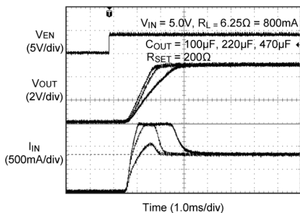
2097 Inrush Current Response
