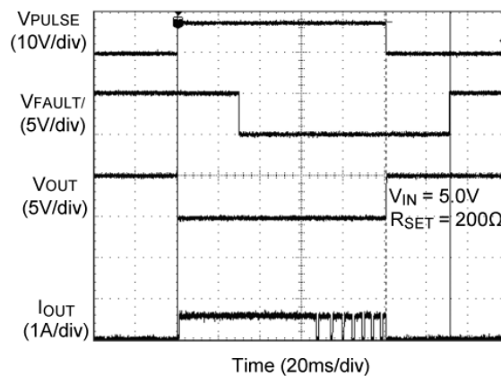
2099 Output Recovery from Thermal Shutdown
