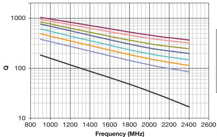
Accu-P® 1210 Typical Q vs Frequency
