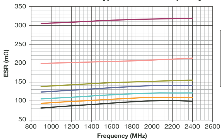
Accu-P® 0805 Typical ESR vs Frequency
