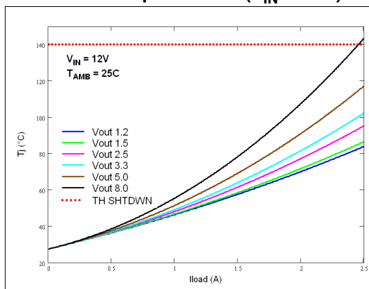
Figure 37. Junction temperature vs. output current ( V_{IN} = 12V )
