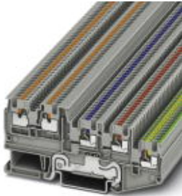
Sensor/actuator terminal block, Connection method: Push-in connection, Cross section: 0.14 mm 2 - 1.5 mm 2 , AWG: 26 - 14, Width: 3.5 mm, Color: gray, Mounting type: NS 35/7,5, NS 35/15
