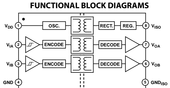
Figure 1. ADuM5240
