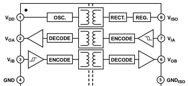
Figure 2. ADuM5241
