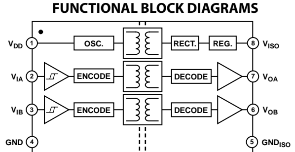
Figure 1. ADuM5240
