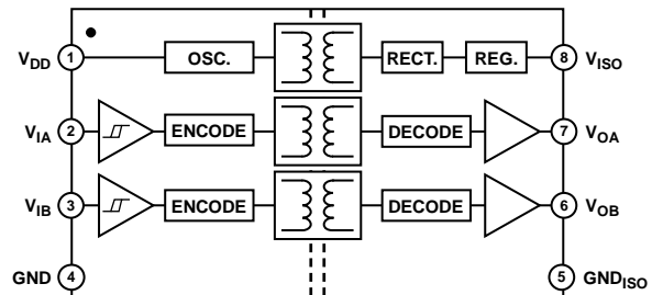
Figure 1. ADuM5240
