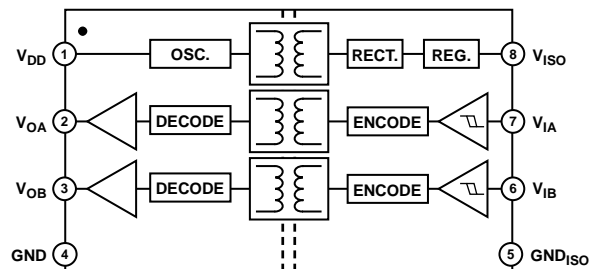
Figure 3. ADuM5242
