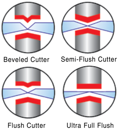
Flush Cutter
