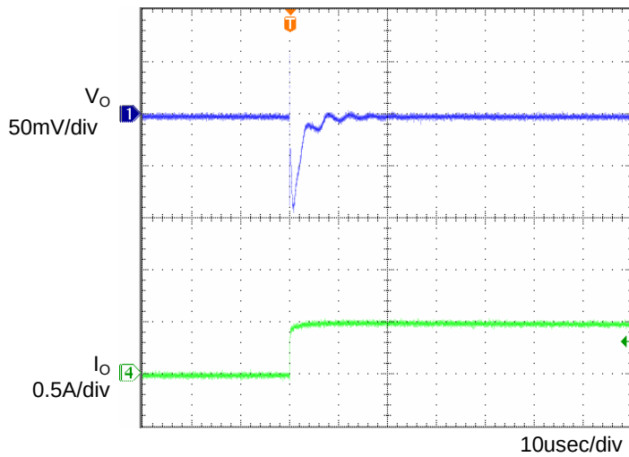
Fig.5 Transient Response (0→0.5A) C_o=1\mu\text{F} , T_a=105^\circ\text{C}
