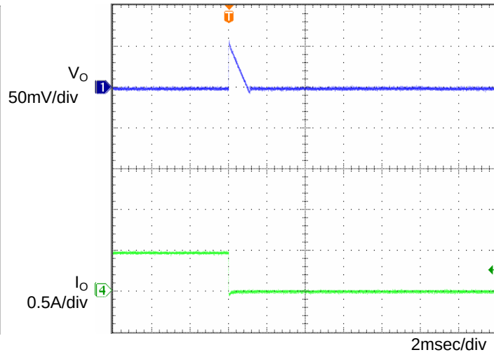
Fig.6 Transient Response (0.5→0A) C_o=1\mu\text{F} , T_a=-40^\circ\text{C}
