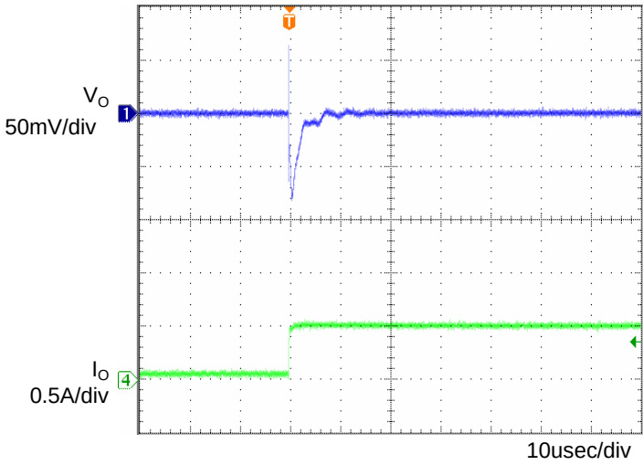
Fig.4 Transient Response (0→0.5A) C_o=1\mu\text{F} , T_a=25^\circ\text{C}
