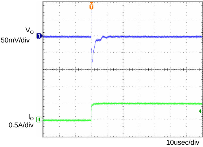
Fig.3 Transient Response (0→0.5A) C_o=1\mu\text{F} , T_a=-40^\circ\text{C}
